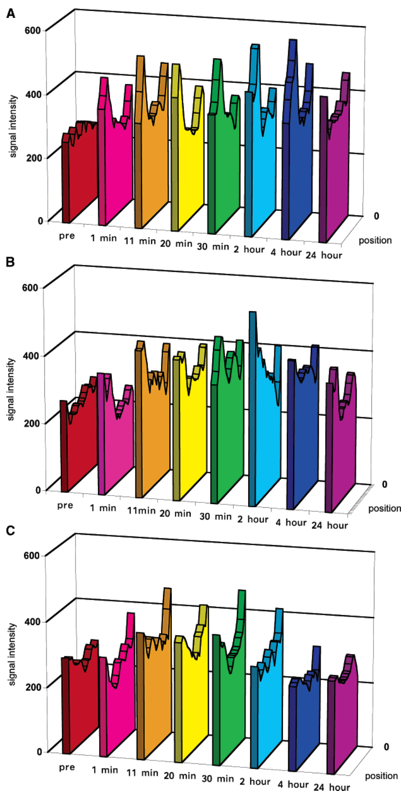
Figure 4. Plot profile of signal intensity through tumor tissues before and at various time points after the injection of PGA-1,6-hexanediamine-(Gd-DO3A) conjugates ((a) 87, (b) 50, and (c) 28 kDa). The cross section positions are indicated by arrow 4 in Figure 1.
