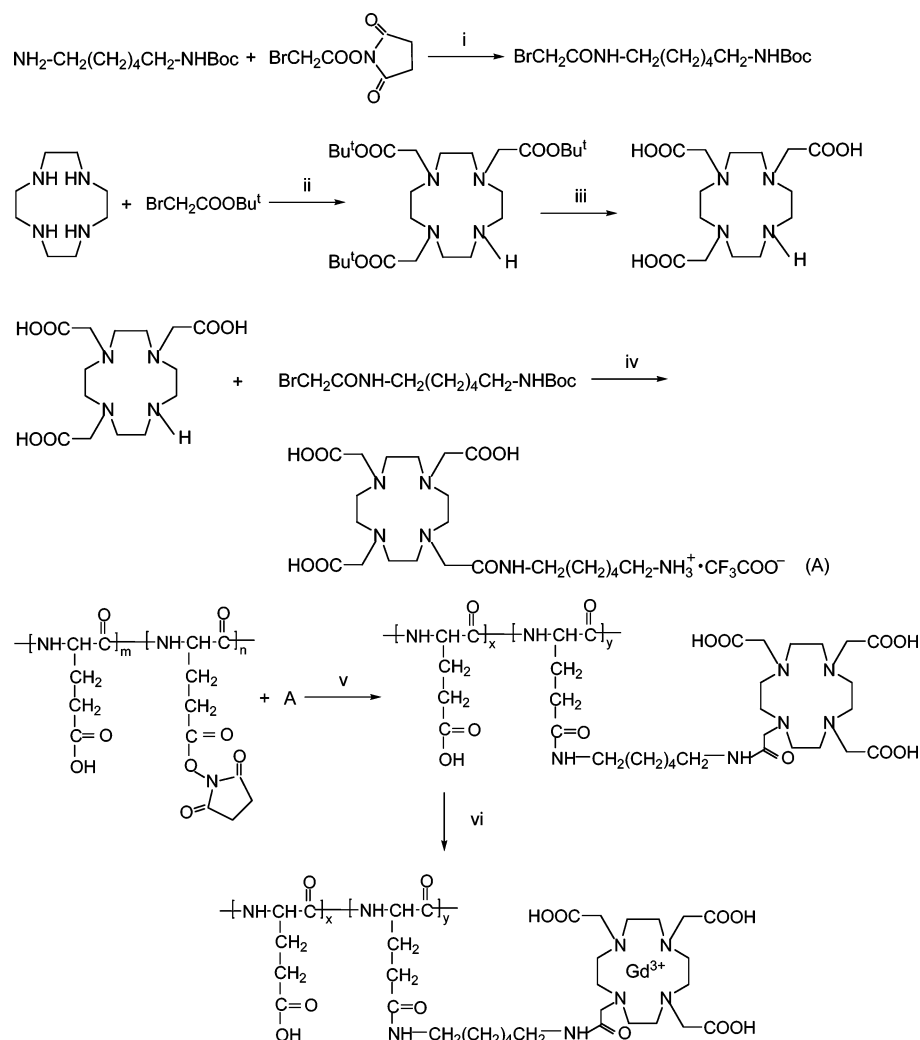
Scheme 1. Synthetic Procedure for PGA-1,6-hexanediamine-(Gd-DO3A) a
